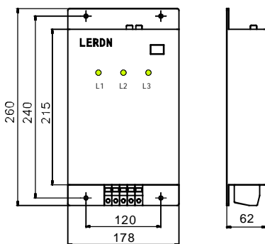
Appearance and installation dimension
