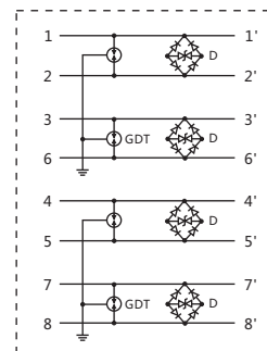
LDY-C/RJ45/SK
