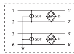
LDY-C/RJ45/S
