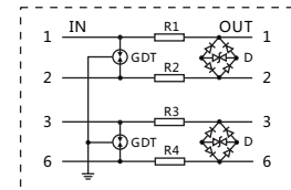
LDY-C/RJ45/L
