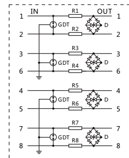
LDY-C/RJ45/LK
